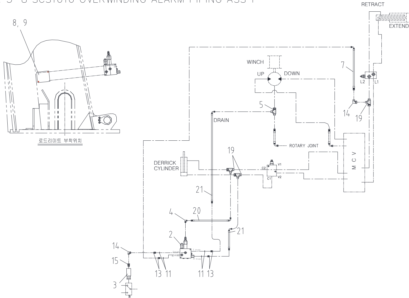
Fig. 5-8 SCS1616 OVERWINDING ALARM PIPING ASS'Y
