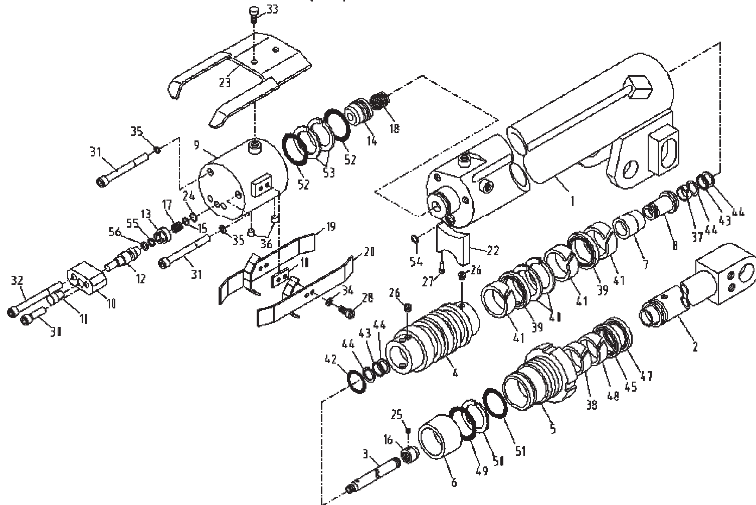
Fig. 1-1-1 SCS1616 TELESCOPIC CYL'(1st) ASS'Y
