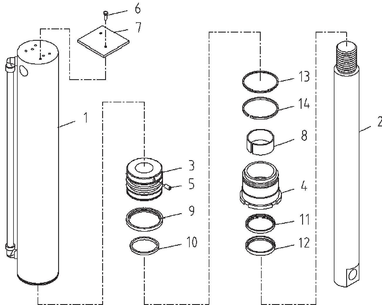
Fig. 9-2-1-1 SCS1616 JACK CYL' ASS'Y
